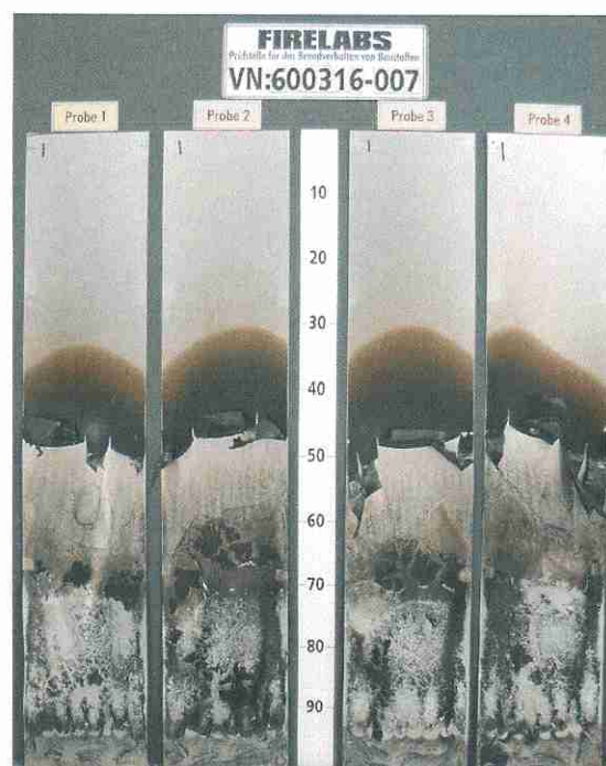
fig. 14 View of test specimen after the test
