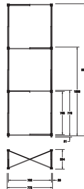
▲ Dimension of a straight system
