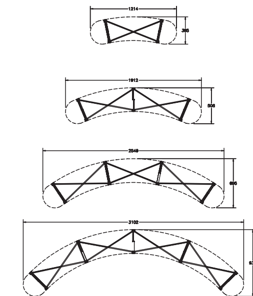
▲ Dimension of a curved system with curved endcaps
