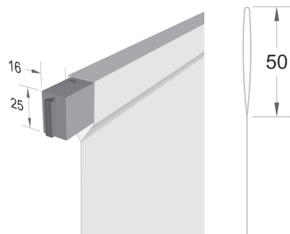
▲ The beam and pocket size for the fabric panel
