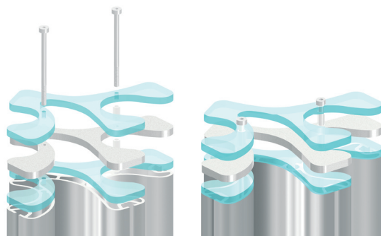
Fastening of an end plate extension kit to the organic upright extrusion
