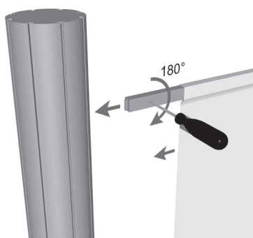
▲ Attach the upper beam, stretch the fabric and lock the lower beam
