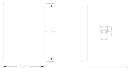
VA 6204 Picture frame, for panel 700x1000mm collapsable, incl. 4 corner connectors
