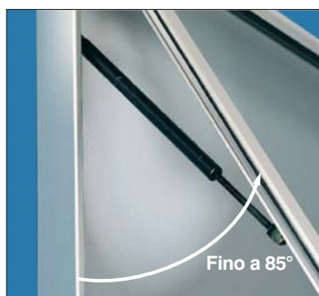
Comoda apertura frontale con stantuffi a gas. Easy opening to an angle of 85° thanks to gas pressure springs.
